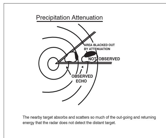
FIG ENR 1.1-21 Limitations to Radar Service
