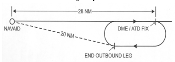
FIG ENR 1.5-5 Inbound Leg Away from NAVAID
