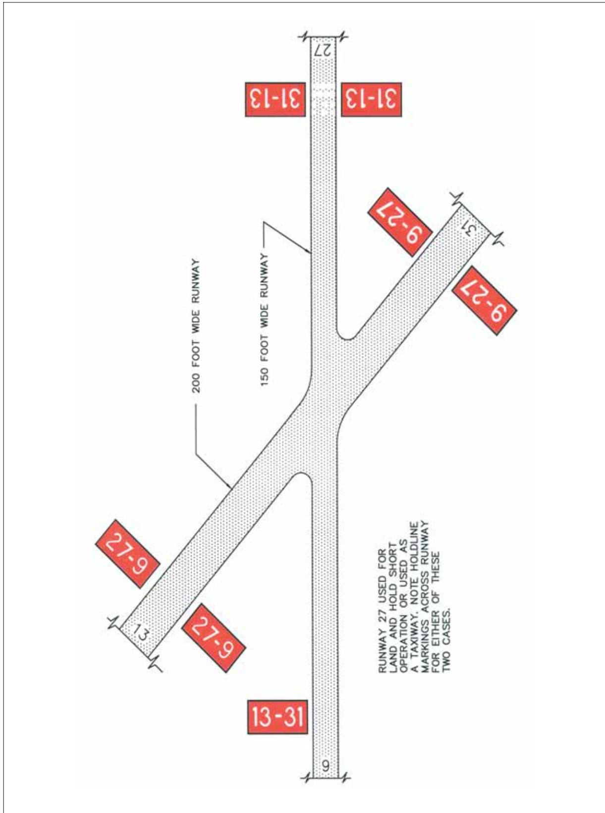
FIG AD 1.1-23 Runway Holding Position Markings on Runways
