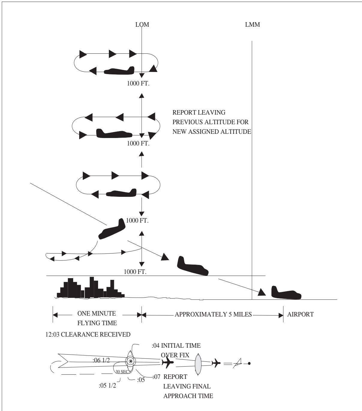
FIG ENR 1.5-30 Timed Approaches from a Holding Fix
