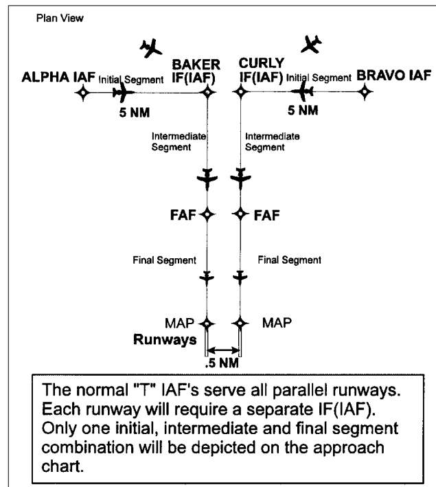
FIG ENR 1.5-15 Modified "T" Approach to Parallel Runways
