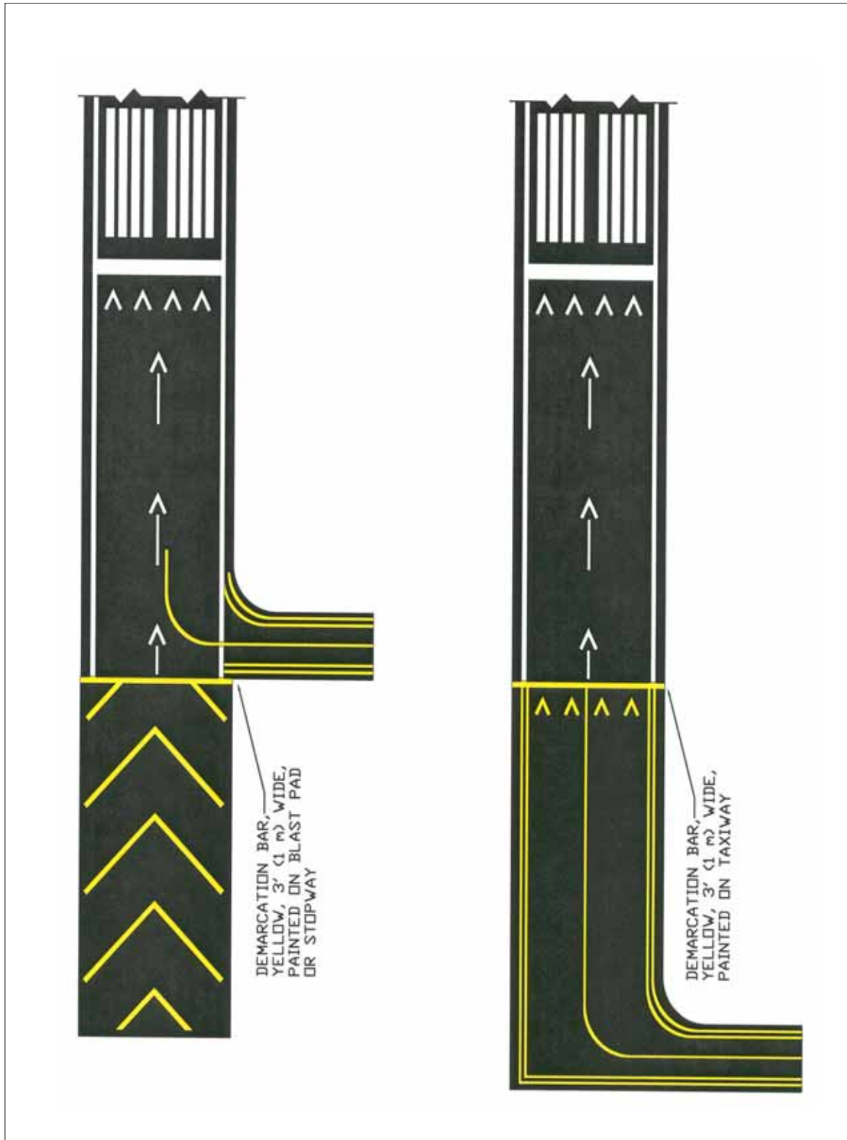
FIG AD 1.1-15 Markings for Blast Pad or Stopway or Taxiway Preceding a Displaced Threshold
