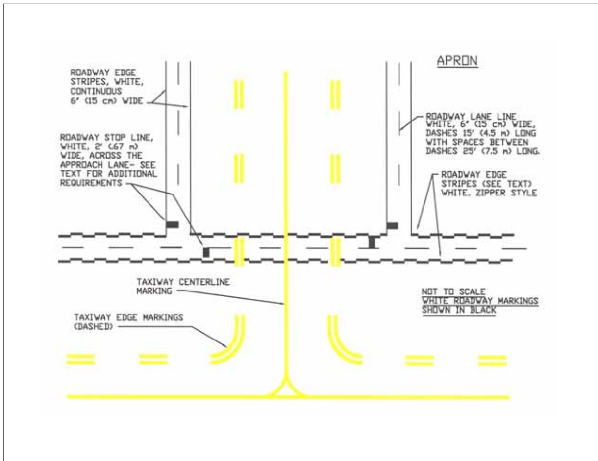
FIG AD 1.1-27 Vehicle Roadway Markings
