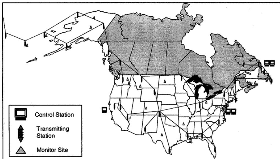
FIG ENR 4.1-6 U.S. and Canadian LORAN System Architecture
