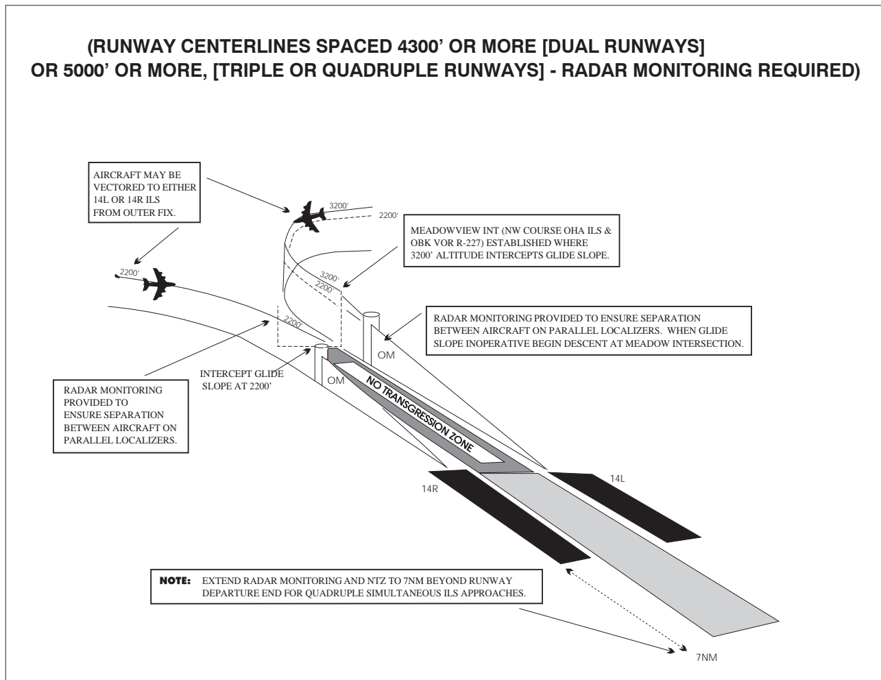
FIG ENR 1.5-27 Simultaneous Parallel ILS Approaches
