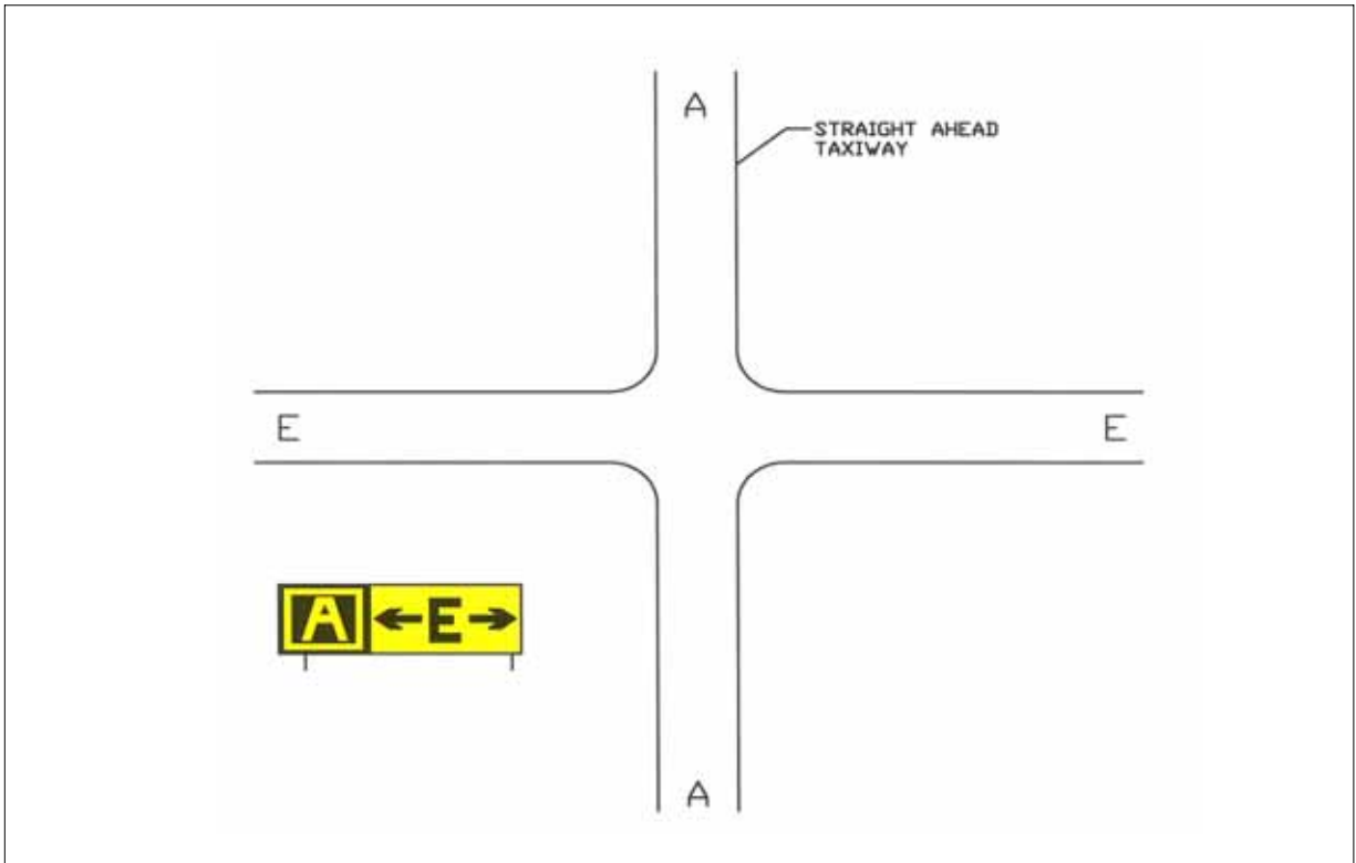
FIG AD 1.1-46 Direction Sign Array for Simple Intersection
