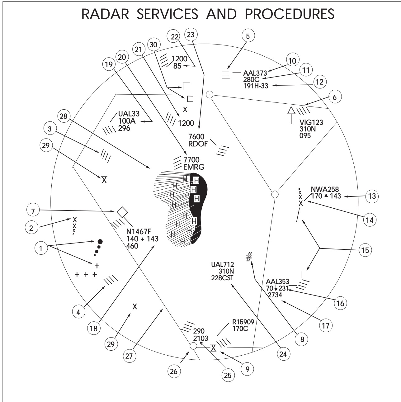
FIG ENR 1.1-23 NAS Stage A Controller's View Plan Display
