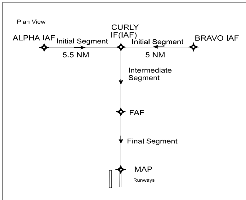
FIG ENR 1.5-17 "T" Approach with Common IAFs to Parallel Runways
