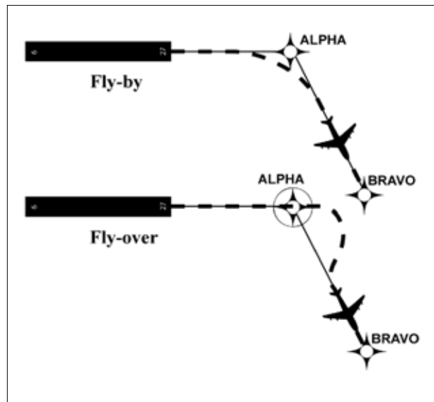
FIG ENR 1.18-1 Fly-by and Fly-over Waypoints
