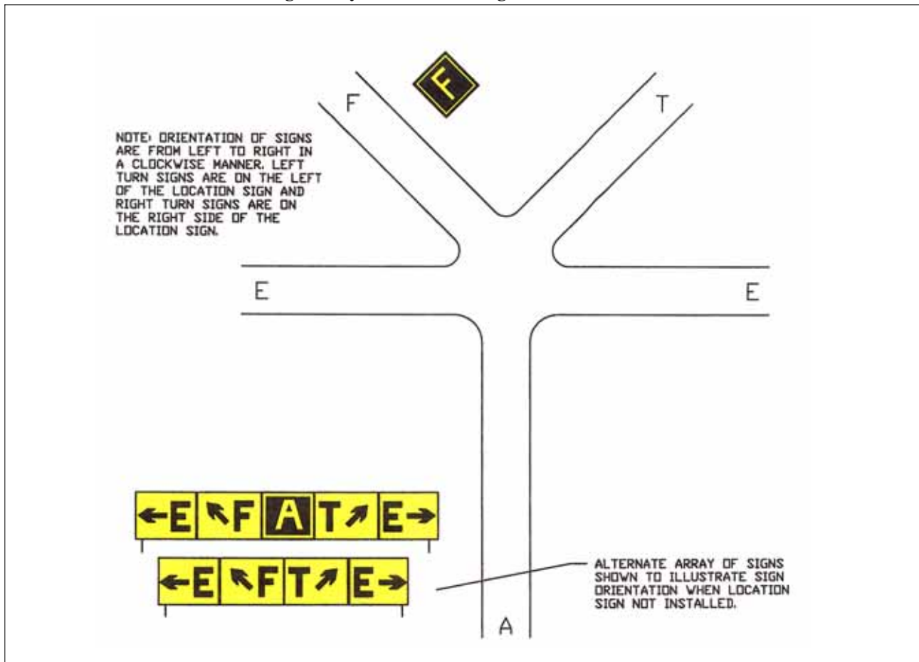
FIG AD 1.1-44 Direction Sign Array with Location Sign on Far Side of Intersection
