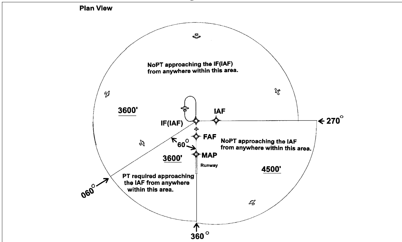
FIG ENR 1.5-22 TAA with Right Base Eliminated
