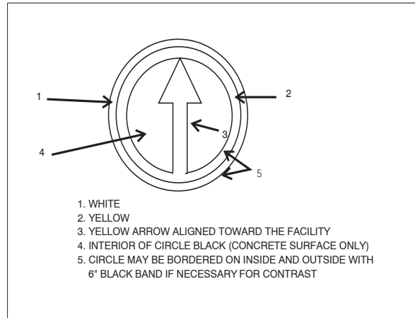
FIG AD 1.1-30 Nonmovement Area Boundary Markings
