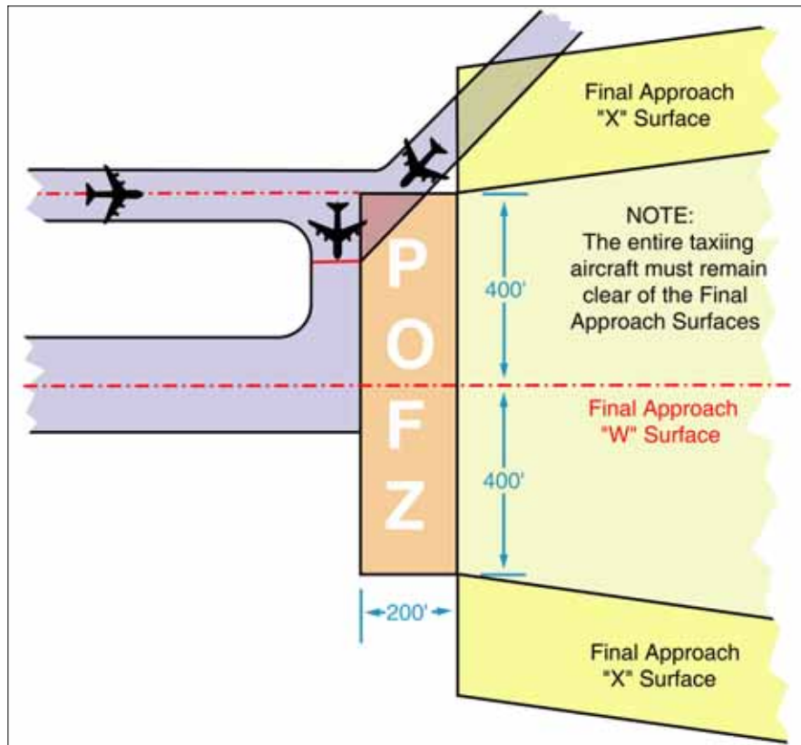
FIG ENR 1.5-11 Precision Obstacle Free Zone (POFZ)
