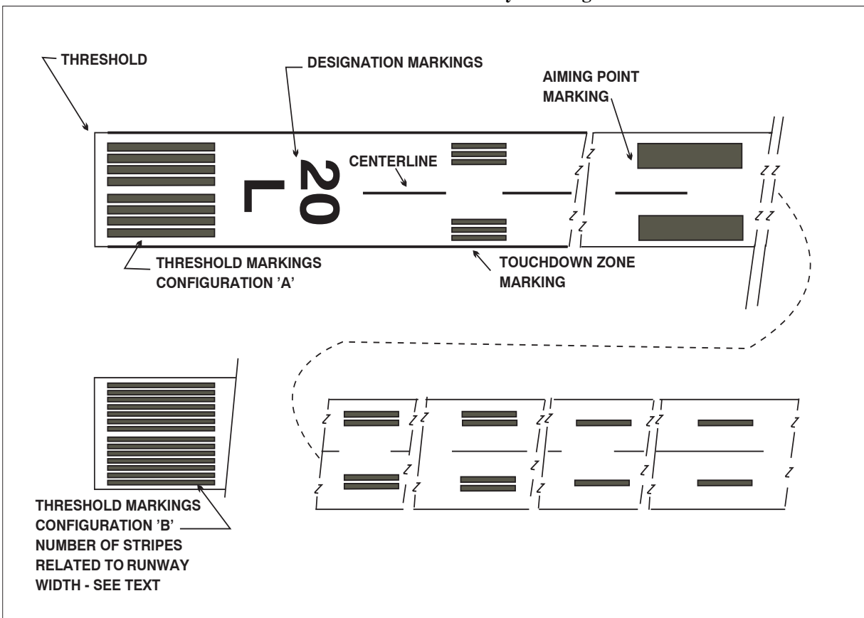
FIG AD 1.1-10 Precision Instrument Runway Markings
