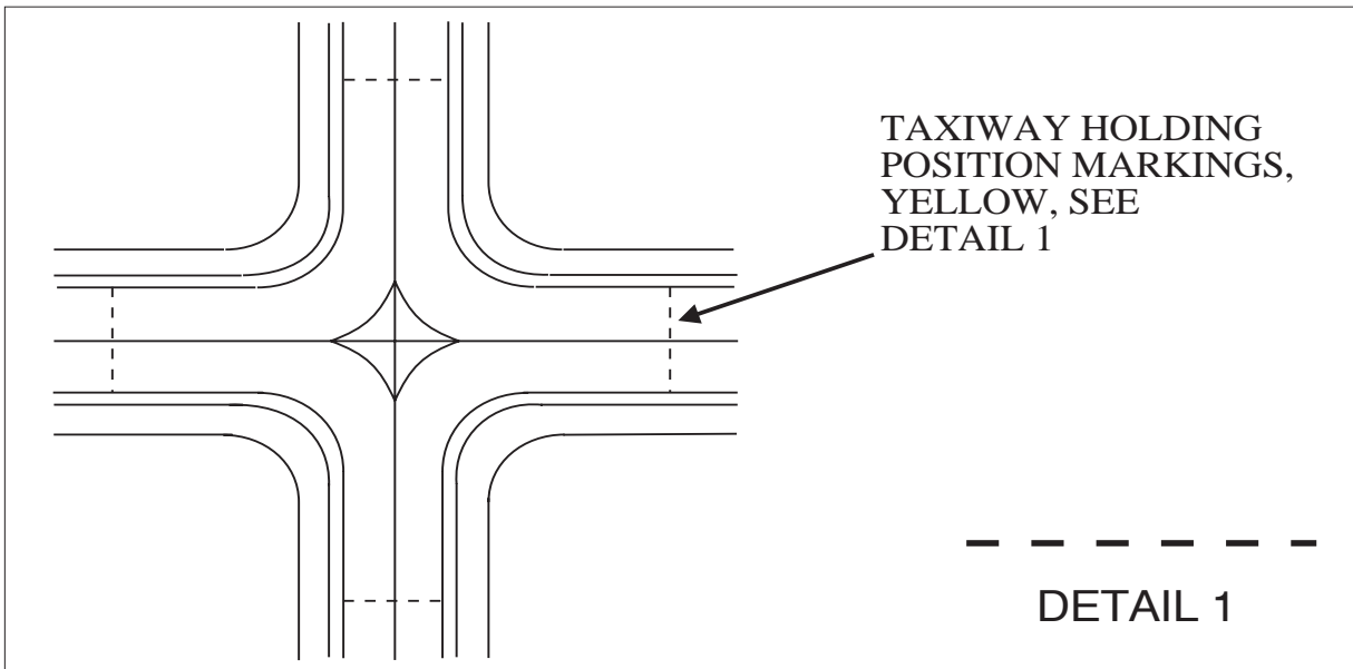
FIG AD 1.1-26 Holding Position Markings: Taxiway/Taxiway Intersections
