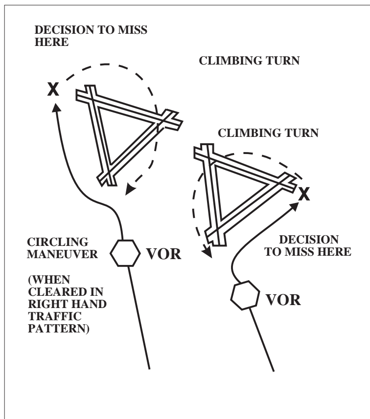
Circling and Missed Approach Obstruction Clearance Areas
