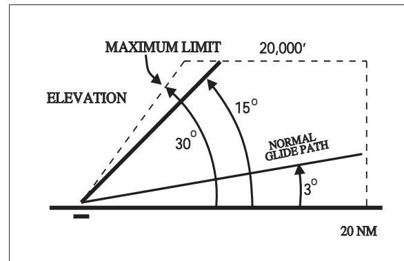
FIG ENR 4.1-4 Coverage Volumes Elevation
