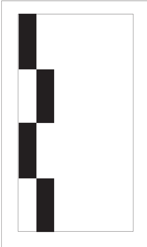
FIG AD 1.1-28 Roadway Edge Stripes, White, Zipper Style
