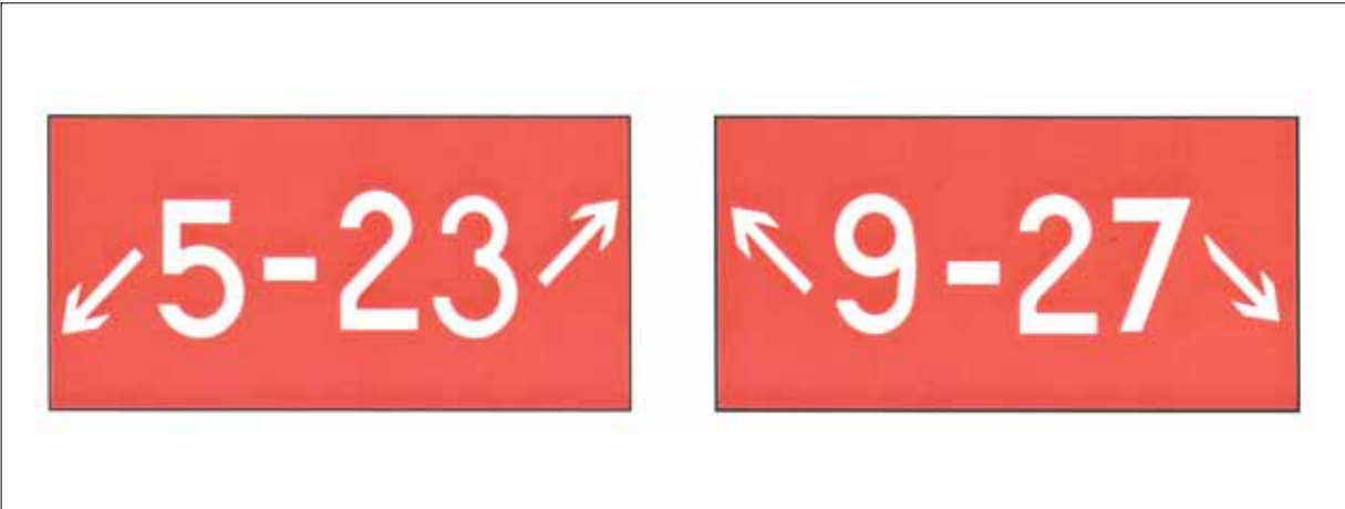
FIG AD 1.1-36 Holding Position Sign for a Runway Approach Area
