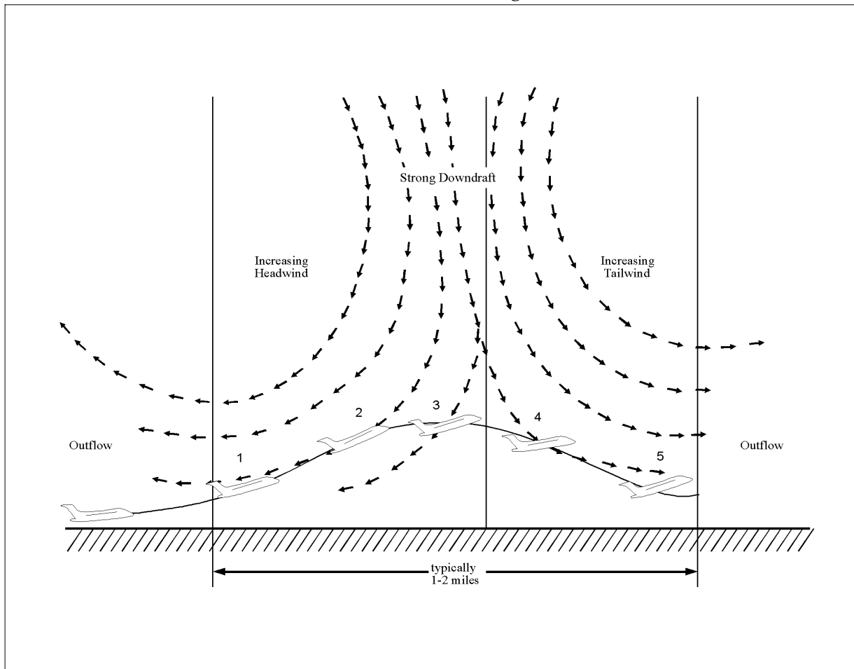
FIG GEN 3.5-11 Microburst Encounter During Takeoff
