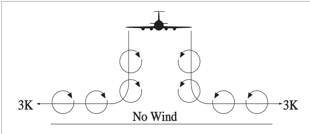
FIG GEN 3.5-22 Vortex Movement Near Ground - No Wind
