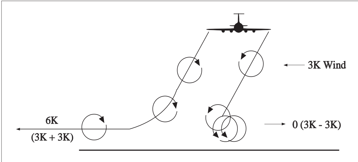
FIG GEN 3.5-23 Vortex Movement Near Ground - with Cross Winds
