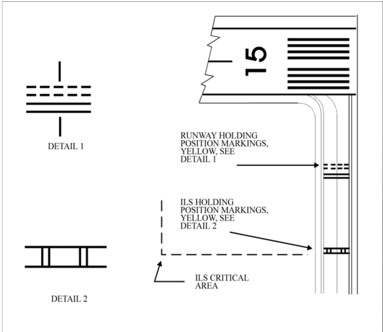
FIG AD 1.1-25 Holding Position Markings: ILS Critical Area
