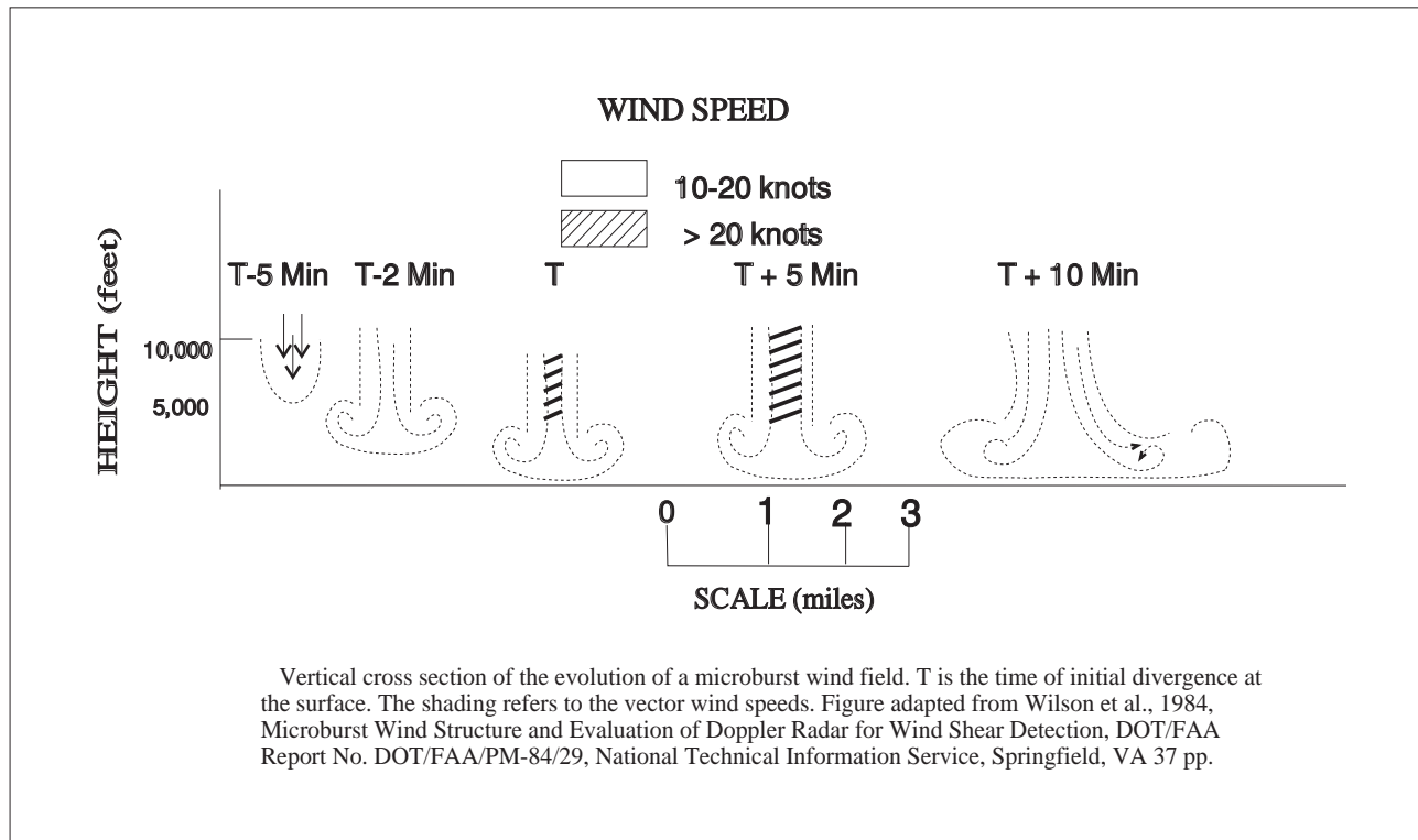
FIG GEN 3.5-10 Evolution of a Microburst
