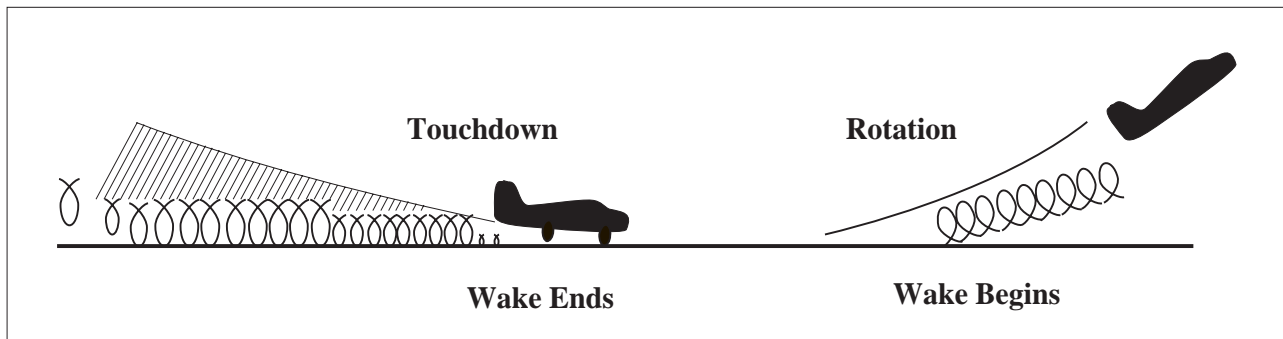
FIG GEN 3.5-20 Wake Ends/Wake Begins
