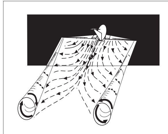
FIG GEN 3.5-18 Wake Vortex Generation
