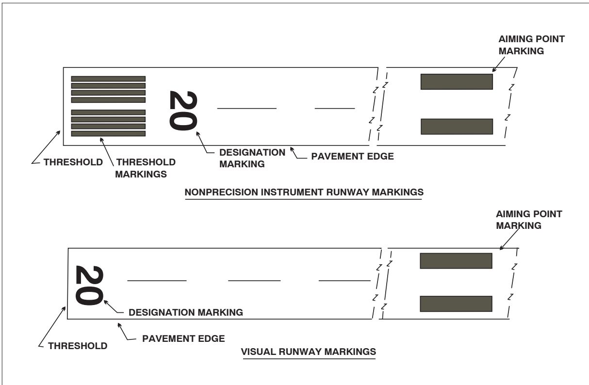
FIG AD 1.1-11 Nonprecision Instrument Runway and Visual Runway Markings
