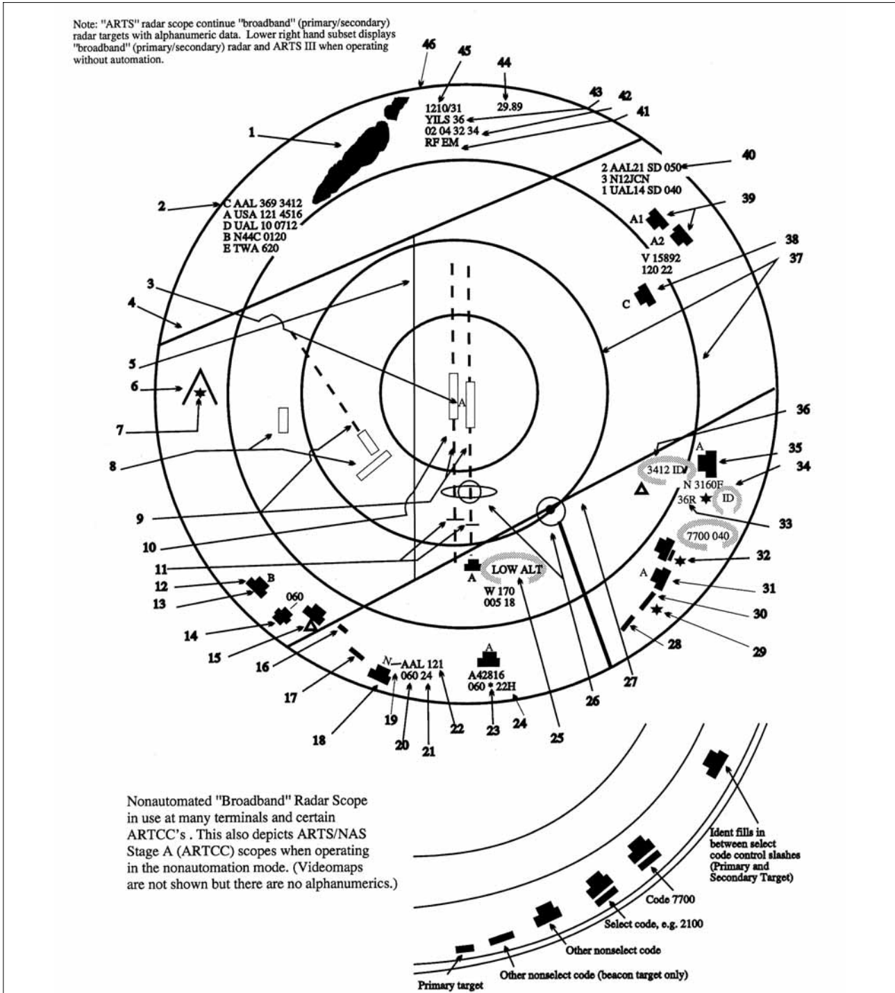
FIG ENR 1.1-22 ARTS III Radar Scope With Alphanumeric Data
