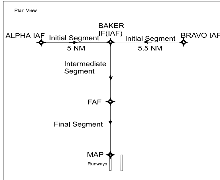
FIG ENR 1.5-16 "T" Approach with Common IAFs to Parallel Runways
