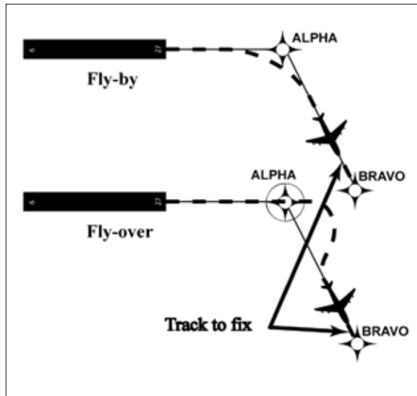
FIG ENR 1.18-2 Track to Fix Leg Type
