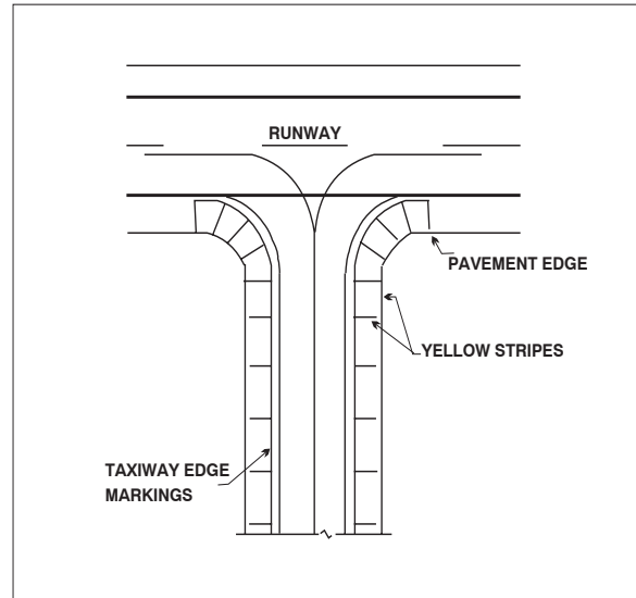
FIG AD 1.1-19 Taxi Shoulder Markings
