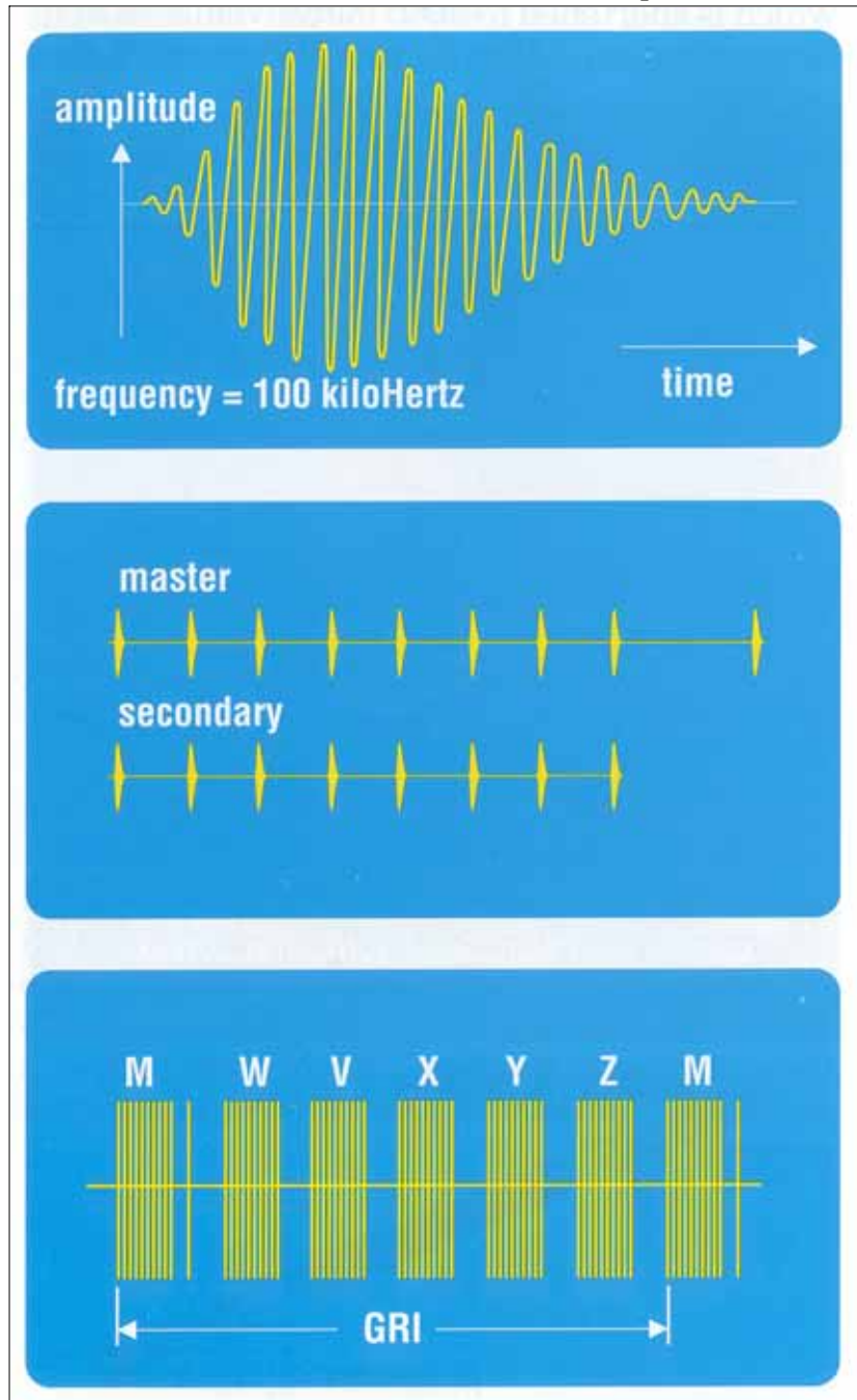
FIG ENR 4.1-8 The LORAN Pulse and Pulse Group
