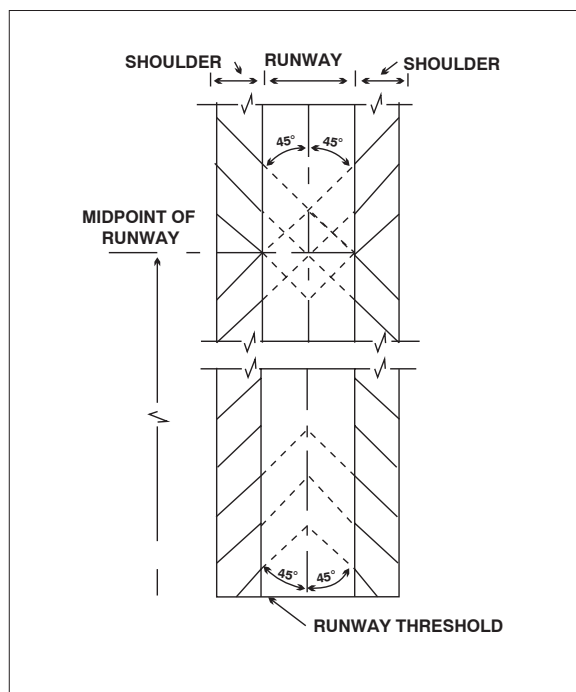
FIG AD 1.1-12 Runway Shoulder Markings
