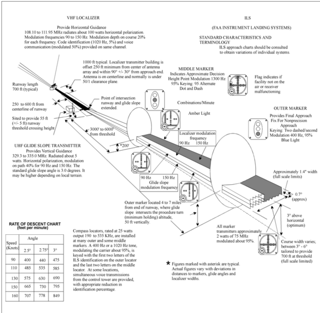
FIG ENR 4.1-2 FAA Instrument Landing Systems
