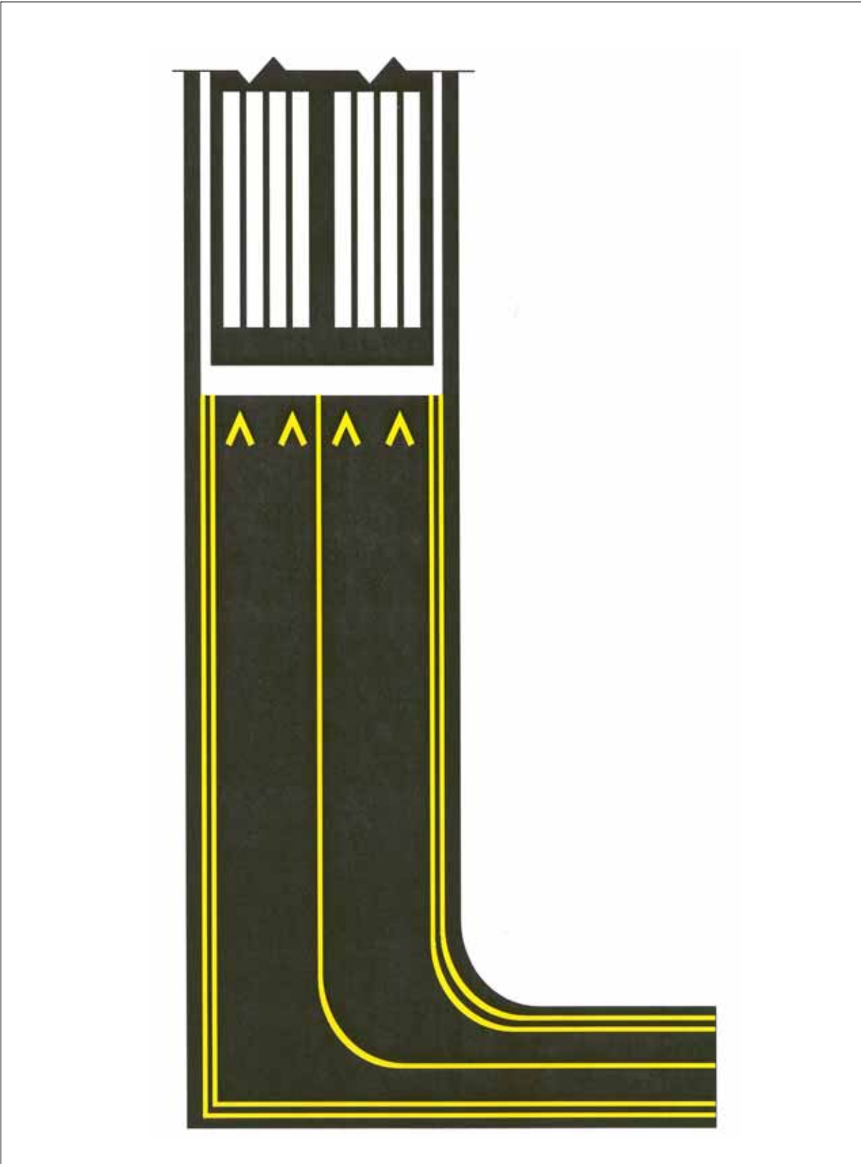
FIG AD 1.1-13 Relocation of a Threshold with Markings for Taxiway Aligned with Runway
