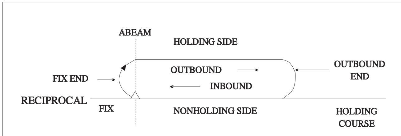
FIG ENR 1.5-2 Holding Pattern Descriptive Terms
