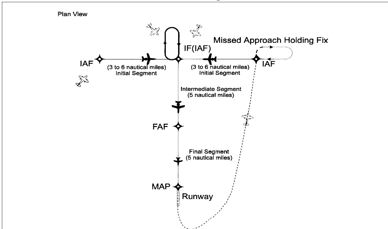
FIG ENR 1.5-13 Basic "T" Design
