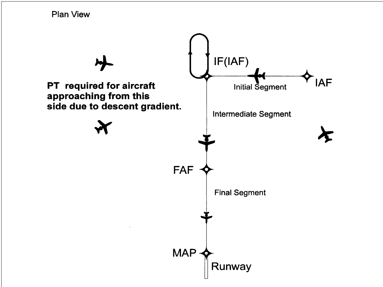
FIG ENR 1.5-14 Modified Basic "T"
