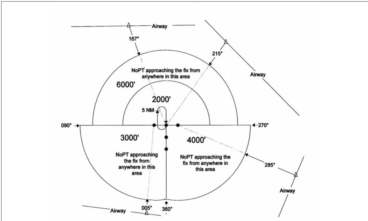
FIG ENR 1.5-23 Examples of a TAA with Feeders from an Airway
