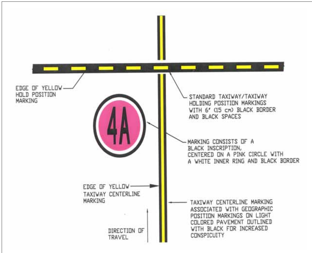
FIG AD 1.1-21 Geographic Position Markings
