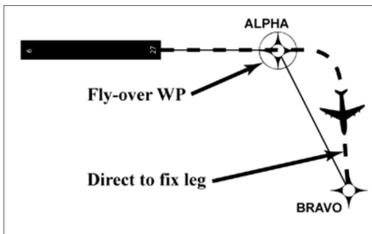
FIG ENR 1.18-3 Direct to Fix Leg Type
