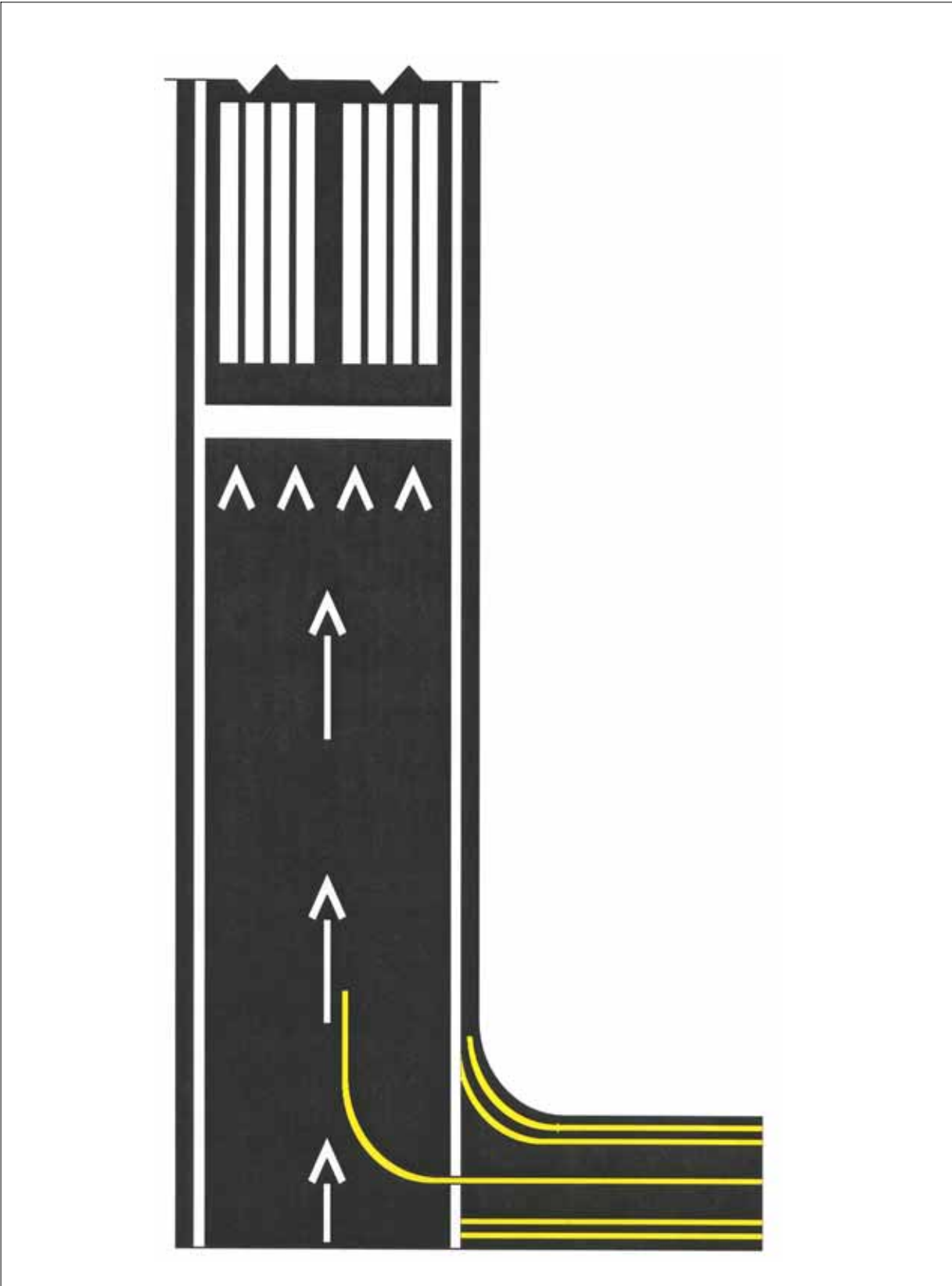
FIG AD 1.1-14 Displaced Threshold Markings
