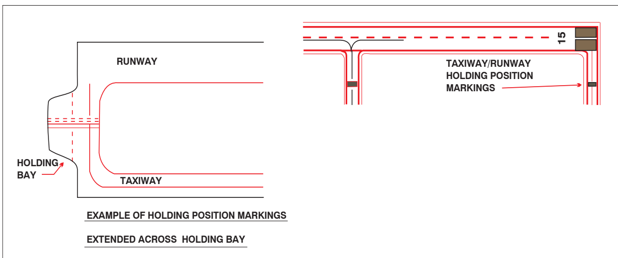
FIG AD 1.1-22 Runway Holding Position Markings on Taxiway
