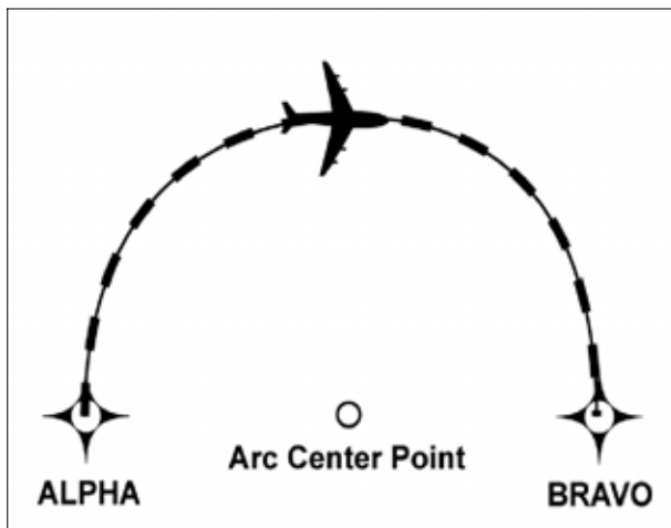
FIG ENR 1.18-5 Radius to Fix Leg Type
