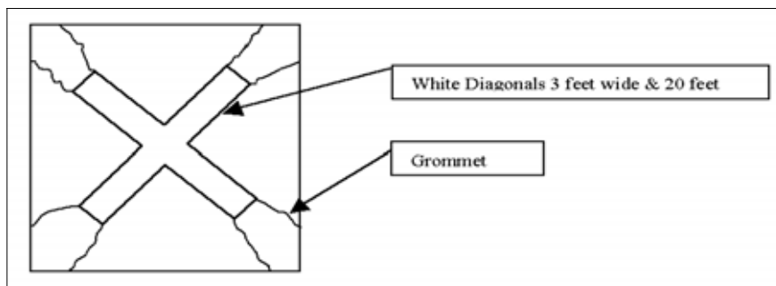
FIG ENR 6.2-2 Closed Helideck Marking
