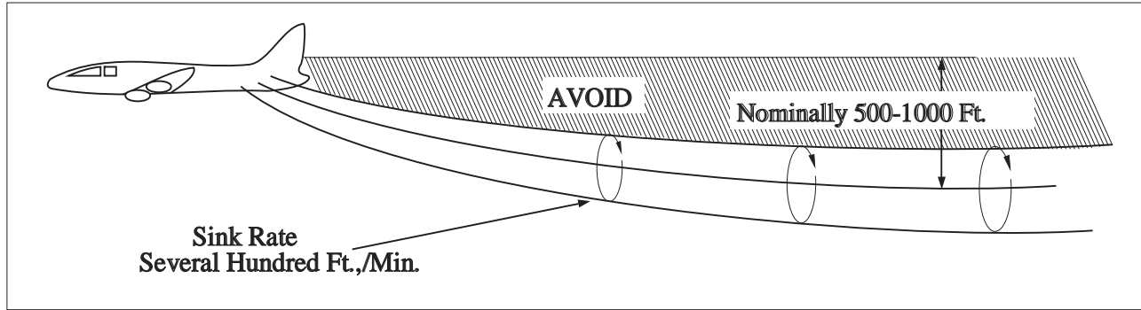
FIG GEN 3.5-21 Vortex Flow Field
