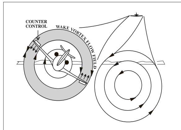
FIG GEN 3.5-19 Wake Encounter Counter Control
