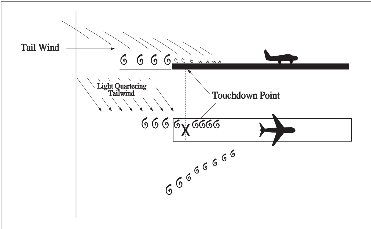
FIG GEN 3.5-24 Vortex Movement in Ground Effect - Tailwind
