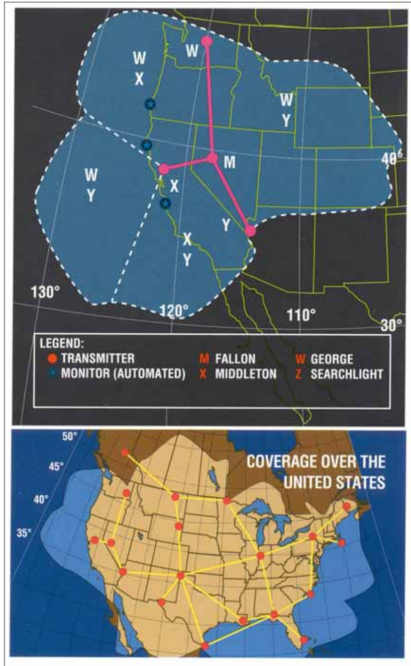
FIG ENR 4.1-10 West Coast U.S. LORAN Chain
