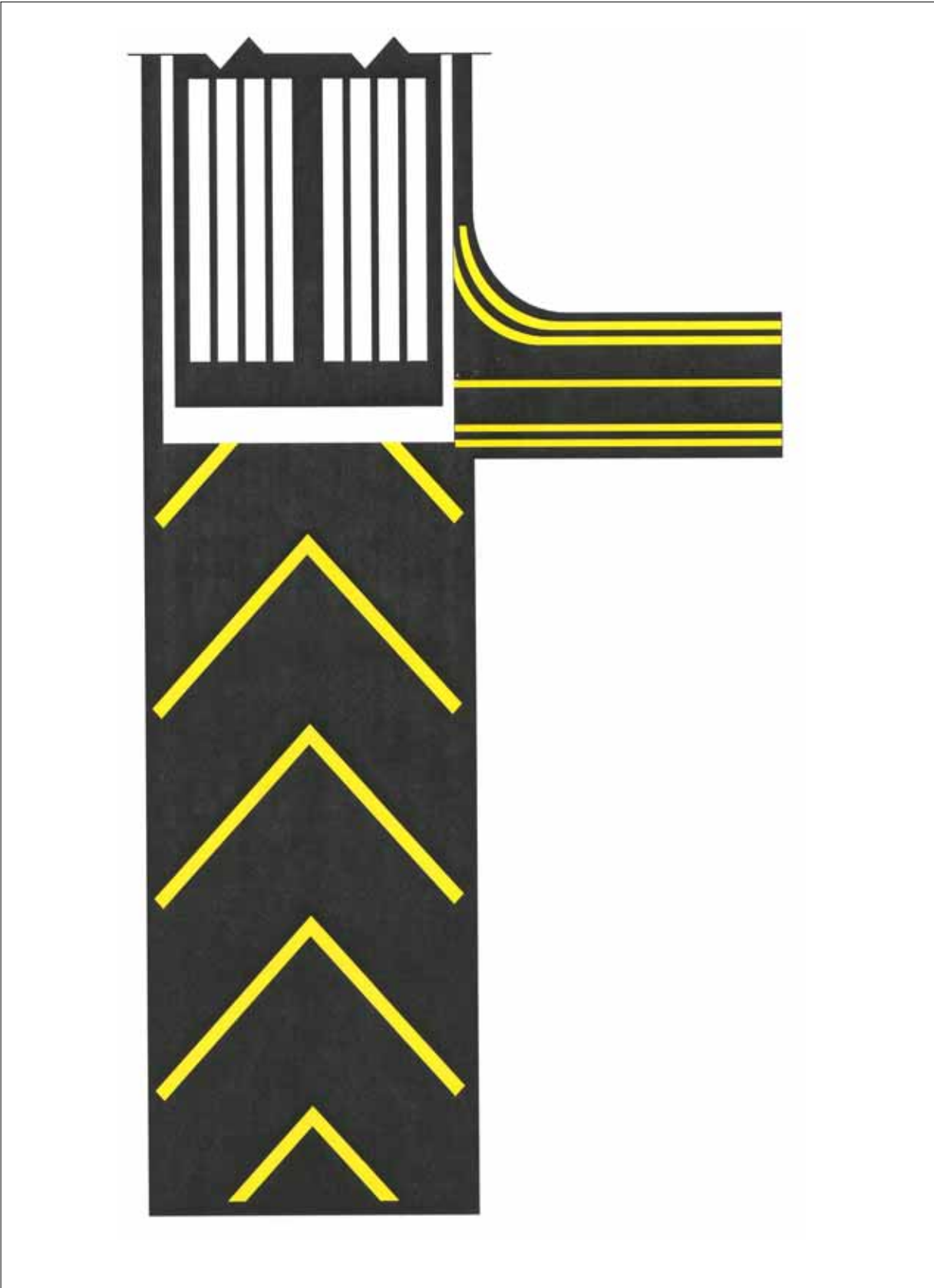
FIG AD 1.1-16 Markings for Blast Pads and Stopways
