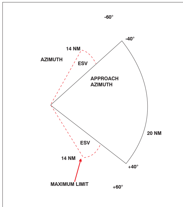
FIG ENR 4.1-3 Coverage Volume Azimuth
