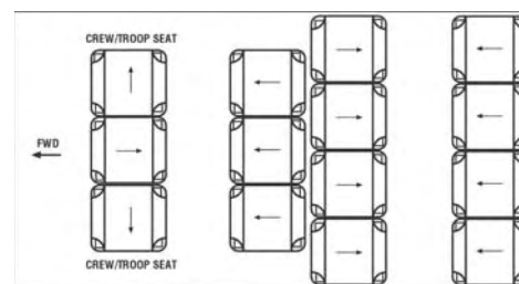
14-passenger cabin
